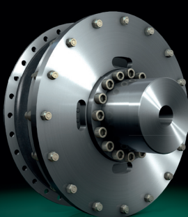
for reasonable misalignment T_{KN} = 1,1 - 25 \text{ kNm}
