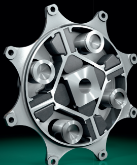
progressive dual stage coupling T_{KN} = 0,15 - 1,75 \text{ kNm}
