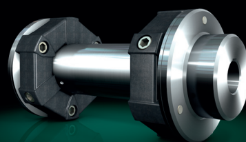
torsional soft flexible shaft for angle up to 2^\circ per element T_{KN} = 0,01 - 12,5 \text{ kNm}
