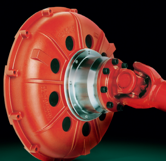
with flexible coupling for u/j T_{KN} = 0,7 - 24 \text{ kNm}
